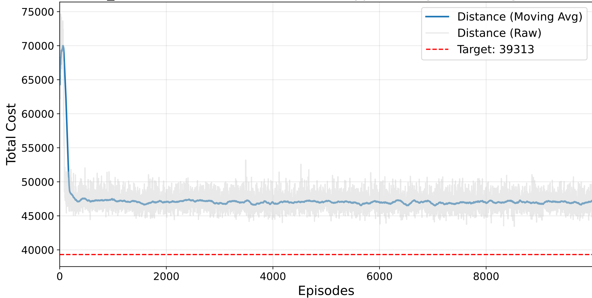
Final NO_BAYESIAN Masked AutoRL-SOP (HyperTuningSK) Training - ft70.1.sop
